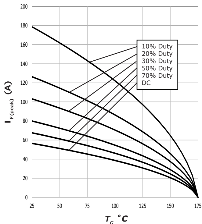
Figure 3. Current Derating
