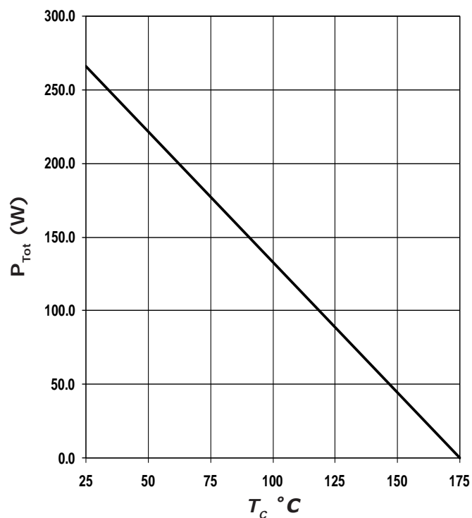
Figure 4. Power Derating
