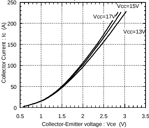
Collector current vs. Collector-Emmitter voltage Tj=125°C
