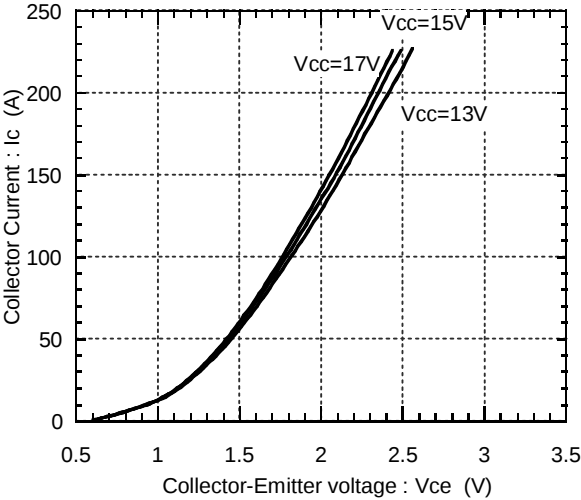
Collector current vs. Collector-Emmitter voltage Tj=25°C
