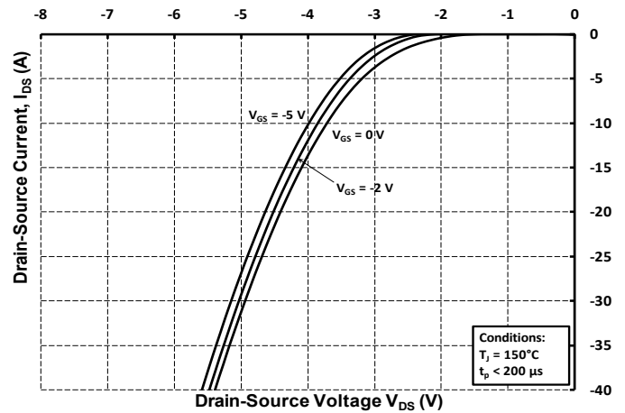
Figure 10. Body Diode Characteristic at 150
