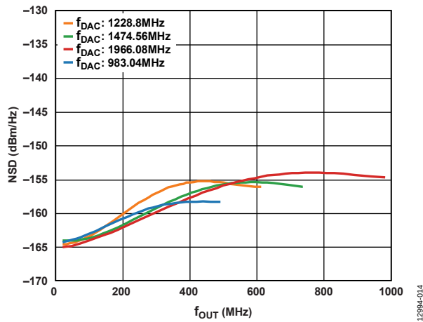
Figure 14. Single Tone (0 dBFS) NSD vs. f_{OUT} over f_{DAC}
