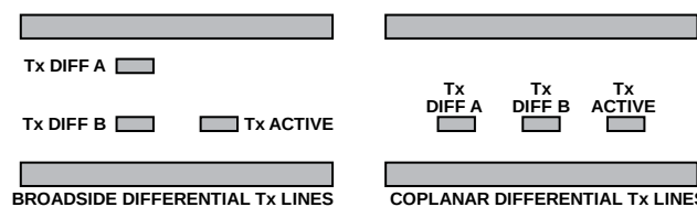
Figure 75. Broadside vs. Coplanar Differential Stripline Routing Techniques
