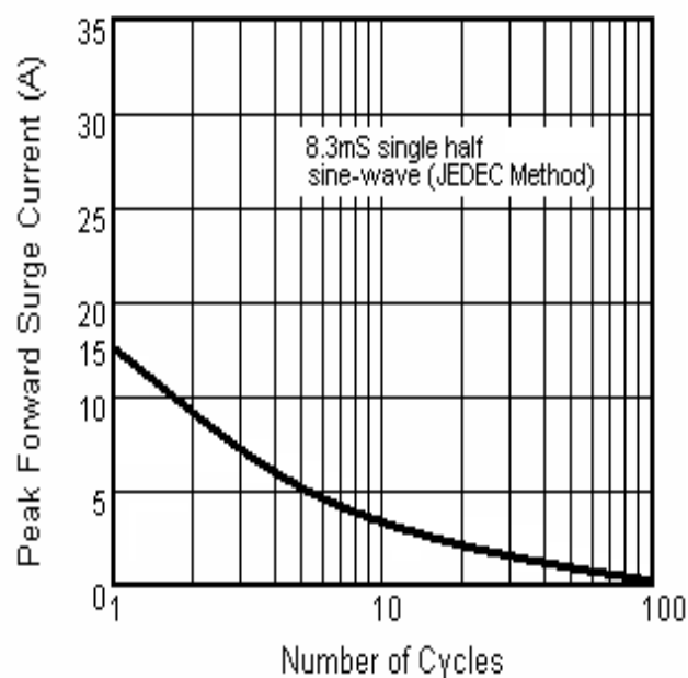
Fig.2 Maximum Non-Repetitive Peak Forward Surge Current
