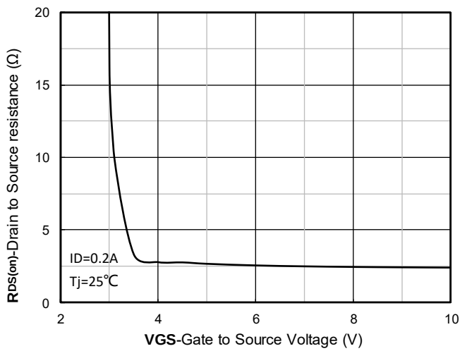
Figure 9. On-Resistance vs Gate to Source Voltage
