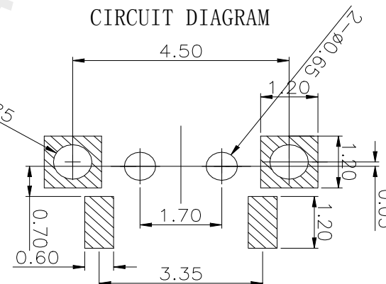
PCB. 焊接图 PCB. WELDING DRAWING
