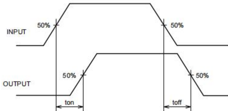
TIMING DIAGRAM
