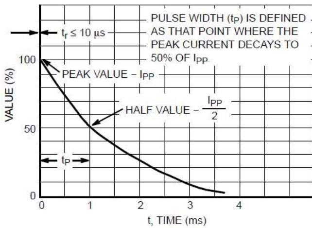
Figure 6. Pulse Waveform
