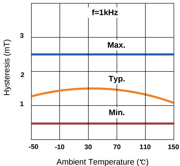
B_{HYS1/2} vs T_A
