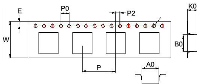
Tape Dimensions
