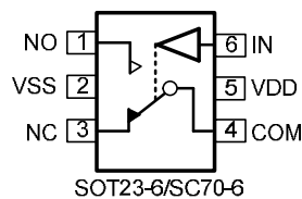
Figure 1. Pin Assignment Diagram
