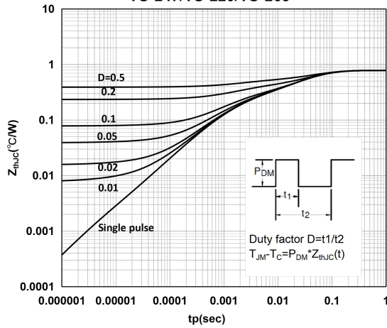
Transient Thermal Response Curve for TO-247/TO-220/TO-263
