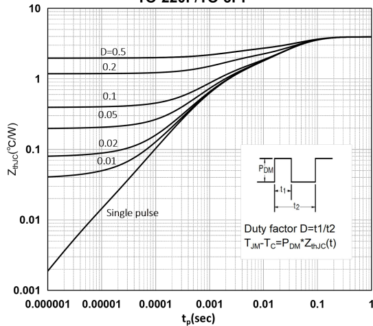
Transient Thermal Response Curve for TO-220F/TO-3PF
