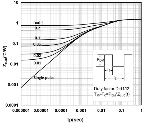
Transient Thermal Response Curve for TO-262
