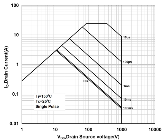
Safe Operating Area for TO-220F/TO-3PF
