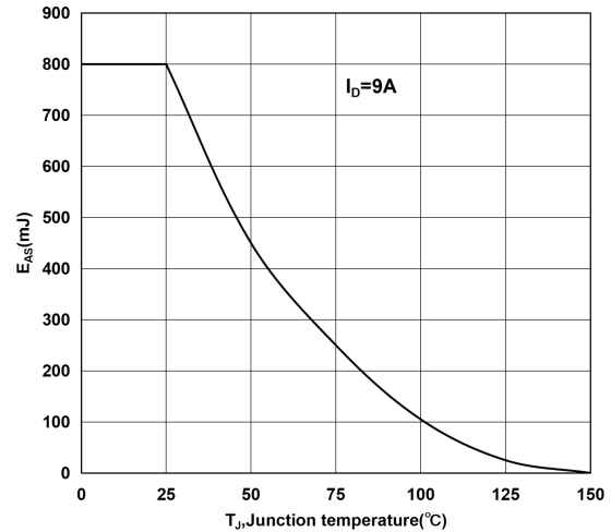
Maximum avalanche energy vs temperature
