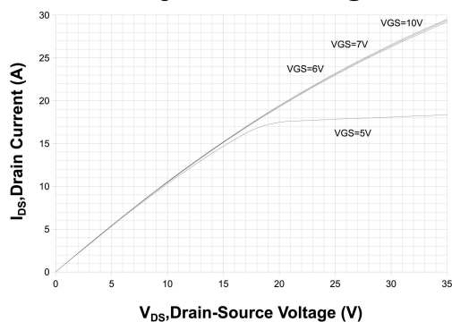
On-Region Characteristics@125°C
