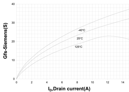
Transconductance
