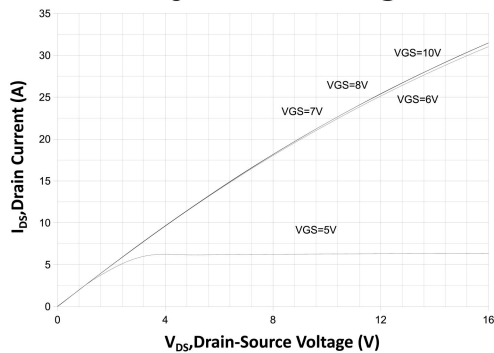
On-Region Characteristics@125°C
