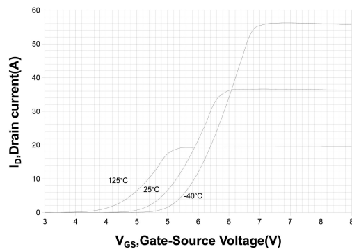
Transfer Characteristics
