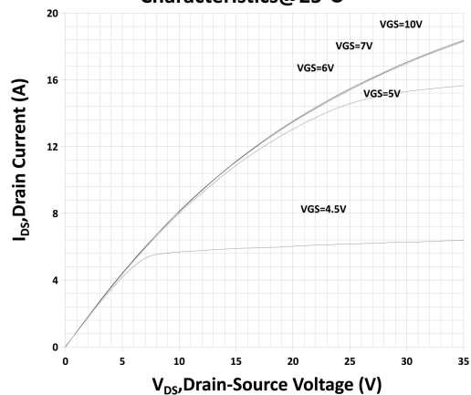
Extended On-Region Characteristics@25°C
