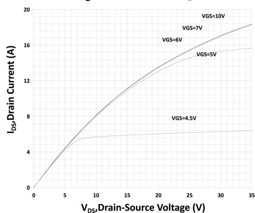
On-Region Characteristics@125°C
