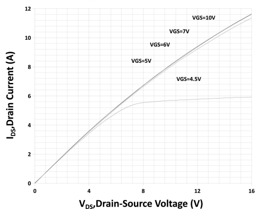
On-Region Characteristics@25°C
