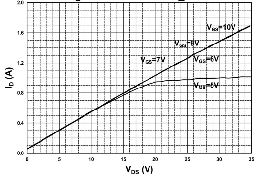
On-Region Characteristics@125°C
