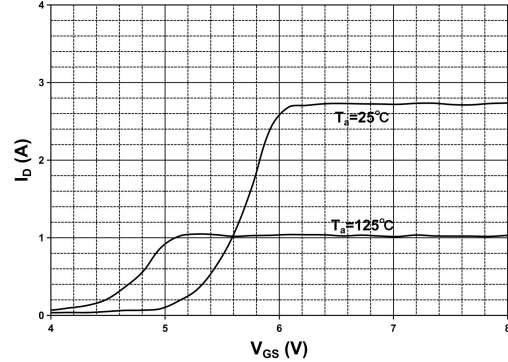
Transfer Characteristics
