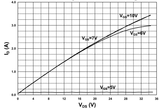
Extended On-Region Characteristic @25°C
