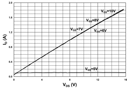
On-Region Characteristics@25°C
