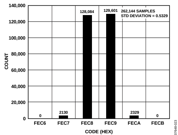
Figure 24. Histogram of 262,144 Conversions of a DC Input at the Code Transition
