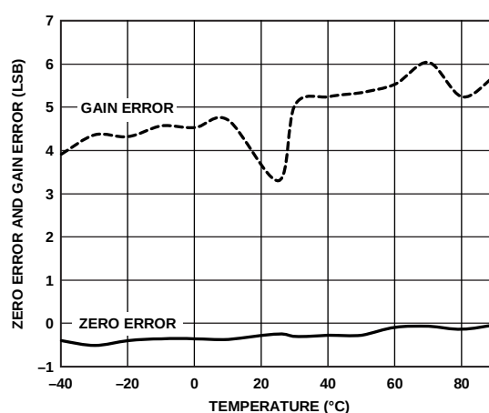
Figure 21. Zero Error and Gain Error vs. Temperature
