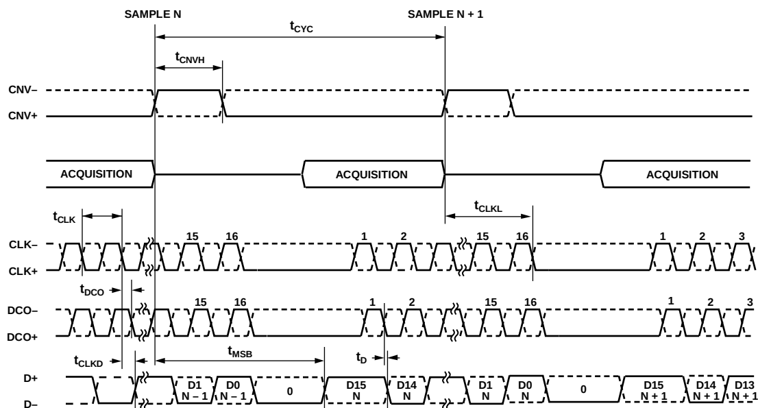
Figure 41. Echoed Clock Interface Mode Timing Diagram
