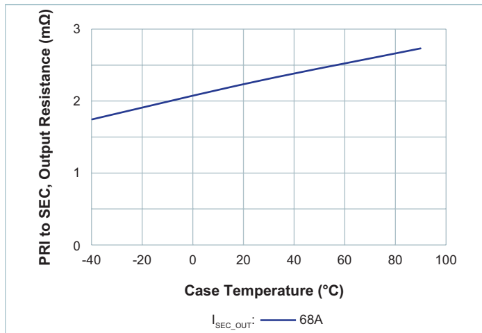
Figure 12 — R_{SEC} vs. temperature; nominal V_{PRI\_DC} I_{SEC\_DC} = 66.67\text{A} at T_{CASE} = 90^{\circ}\text{C}
