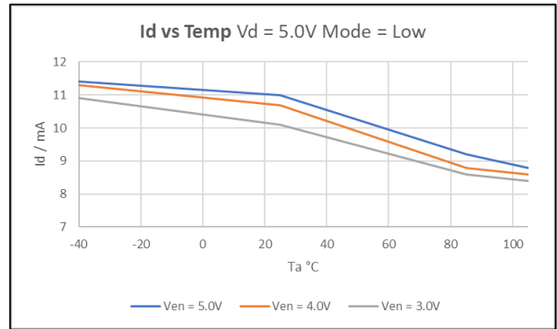
Figure 56: Id v Temp Vd = 5.0V, low current mode
