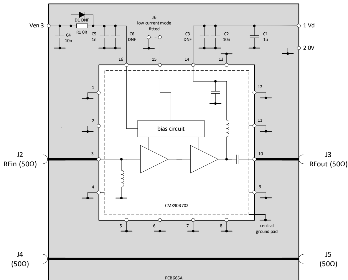
Figure 62: EV90B702 Schematic
