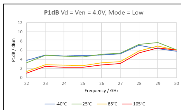
Figure 52: P1dB Vd = Ven = 4.0V, low current mode
