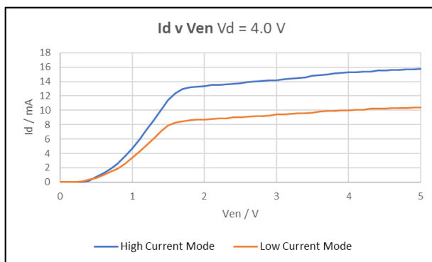
Figure 11: I_d v V_{en} V_d = 4.0V
