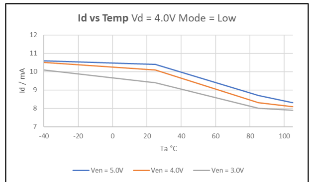
Figure 58: Id v Temp Vd = 4.0V, low current mode
