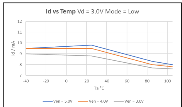
Figure 60: Id v Temp, Vd = 3.0V, low current mode
