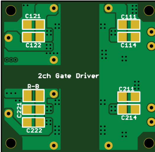
Silkscreen (Bottom)
