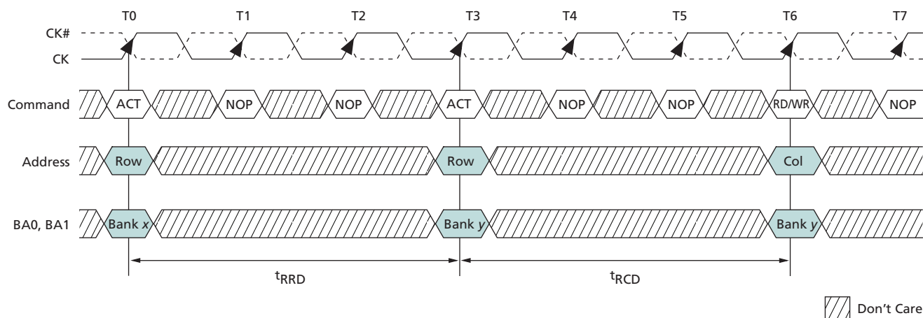
Figure 26: Example: Meeting t_{\text{RCD}} ( t_{\text{RRD}} ) MIN When 2 < t_{\text{RCD}} (t_{\text{RRD}}) \text{ MIN} / t_{\text{CK}} \leq 3
