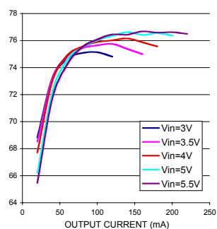
MIC2295 SEPIC 5V Output
