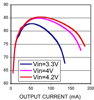
MIC2295 15V output Efficiency
