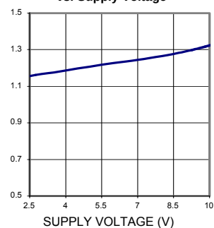
Input Voltage vs. Supply Voltage
