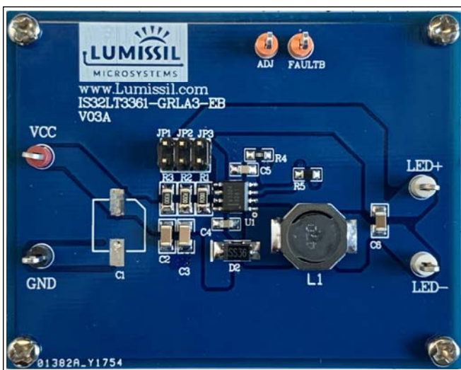
Figure 1 Photo of IS32LT3361 Evaluation Board
