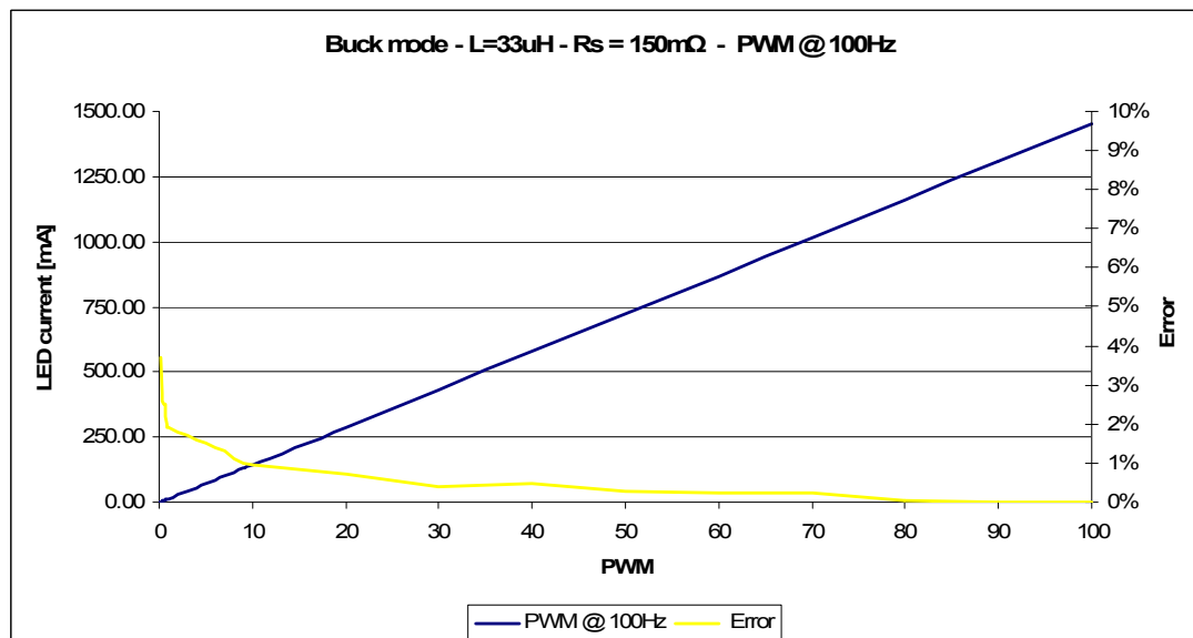
Figure 11. LED Current Linearity and Accuracy with PWM Dimming at 100Hz
