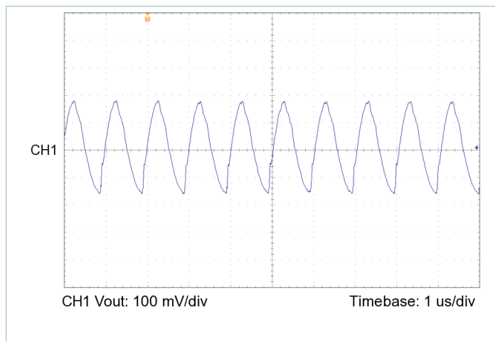
Figure 17 — Output voltage ripple, V_{IN} = 270\text{ V} , V_{OUT} = 24.0\text{ V} , C_{OUT\_EXT} = 220\text{ }\mu\text{F} , R_{LOAD} = 1.152\text{ }\Omega
