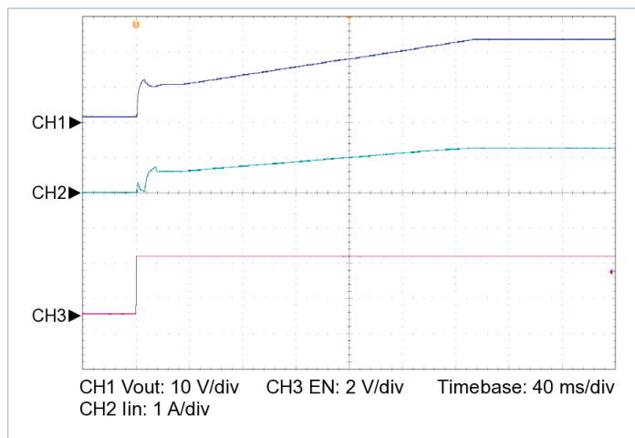
Figure 15 — Startup from EN, V_{IN} = 270\text{ V} , C_{OUT\_EXT} = 2200\text{ }\mu\text{F} , R_{LOAD} = 1.152\text{ }\Omega
