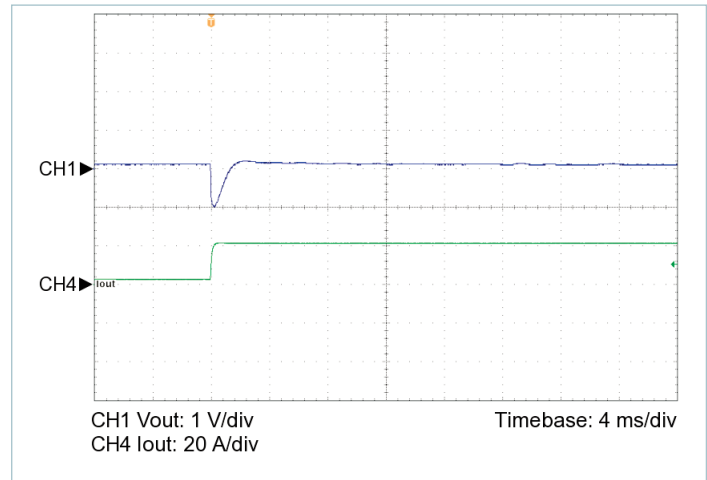
Figure 6 — 10% to 100% load transient response, V_{IN} = 270\text{ V} , nominal trim, C_{OUT\_EXT} = 220\text{ }\mu\text{F}
