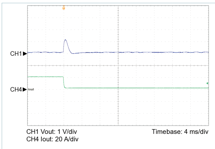
Figure 5 — 100% to 10% load transient response, V_{IN} = 270\text{ V} , nominal trim, C_{OUT\_EXT} = 220\text{ }\mu\text{F}
