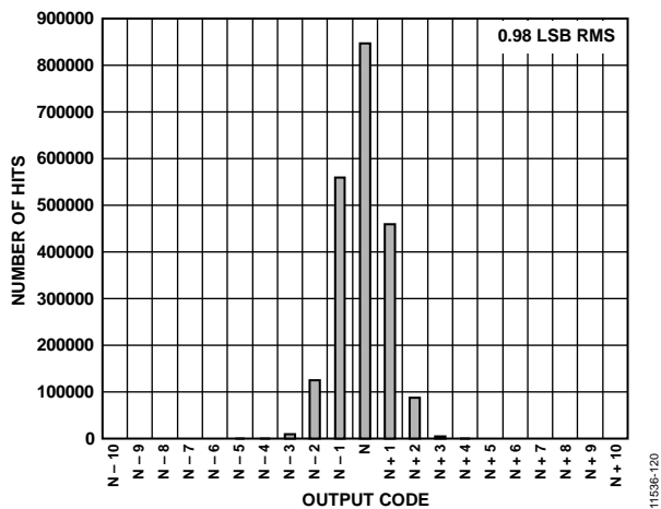
Figure 21. Input Referred Noise Histogram; f_{SAMPLE} = 65 MSPS
