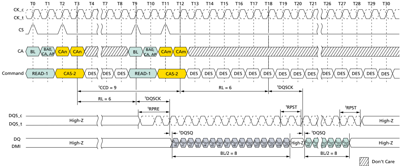
Figure 110: Seamless READ: t_{\text{CCD}} = \text{MIN} + 1 , Preamble = Toggle, 1.5nCK Postamble
