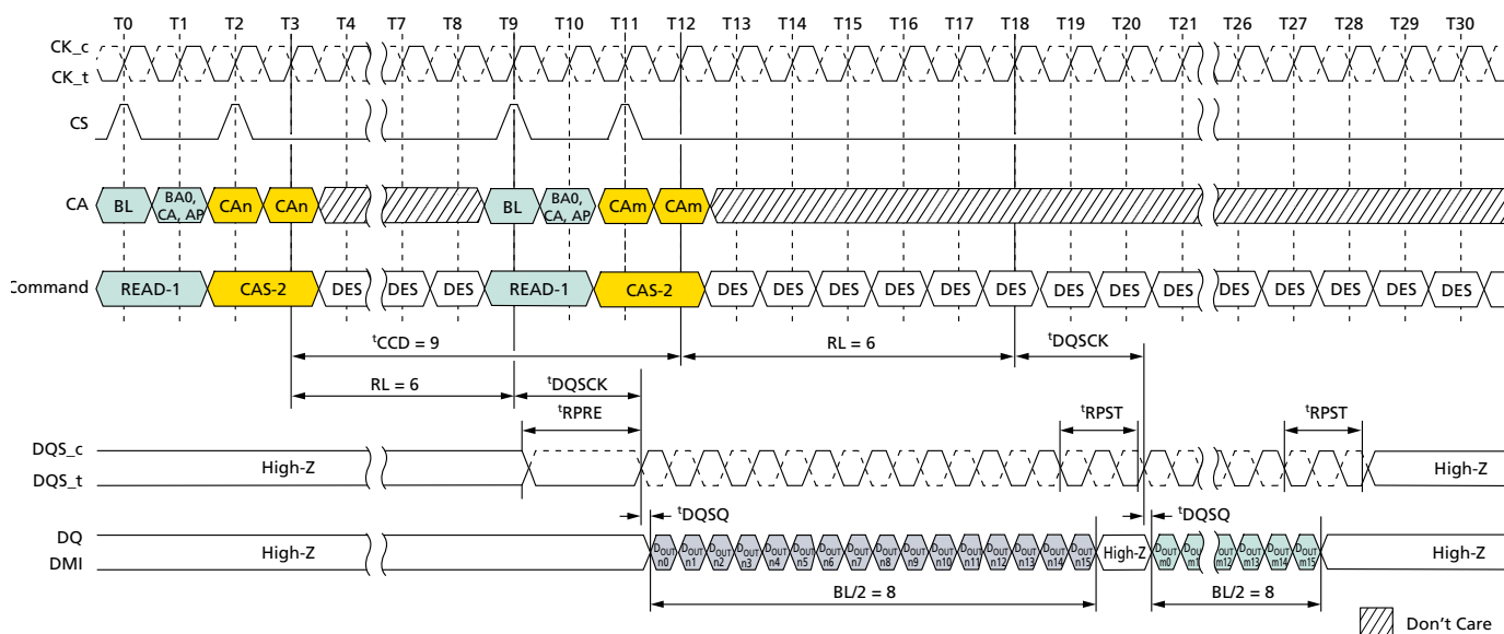
Figure 112: Consecutive READ: t_{CCD} = \text{MIN} + 1 , Preamble = Static, 1.5nCK Postamble
