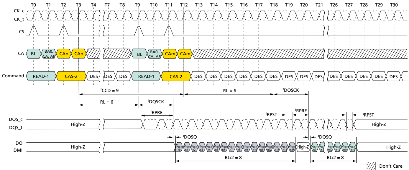
Figure 111: Consecutive READ: t_{\text{CCD}} = \text{MIN} + 1 , Preamble = Toggle, 0.5nCK Postamble
