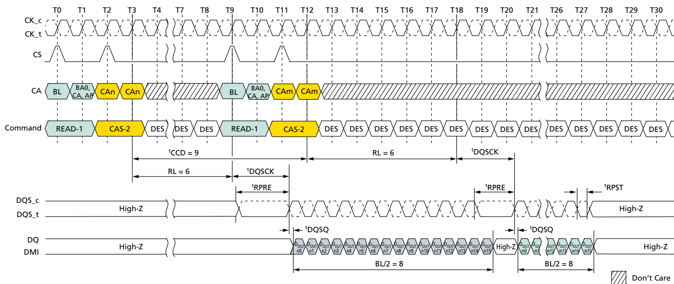
Figure 113: Consecutive READ: t_{CCD} = \text{MIN} + 1 , Preamble = Static, 0.5nCK Postamble
