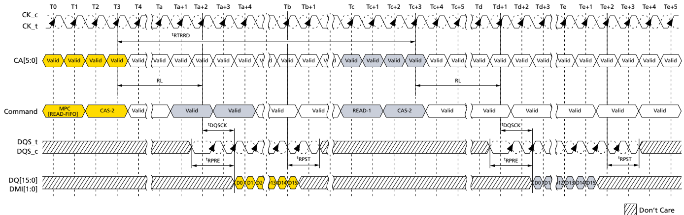
Figure 192: READ-FIFO – t_{\text{RPRE}} = \text{Toggle} , t_{\text{RPST}} = 1.5n\text{CK}
