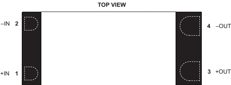
4414PFM VIA - PCB Mount - Pins Down
