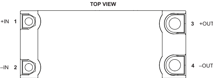
4414PFM VIA - Chassis Mount - Terminals Up
