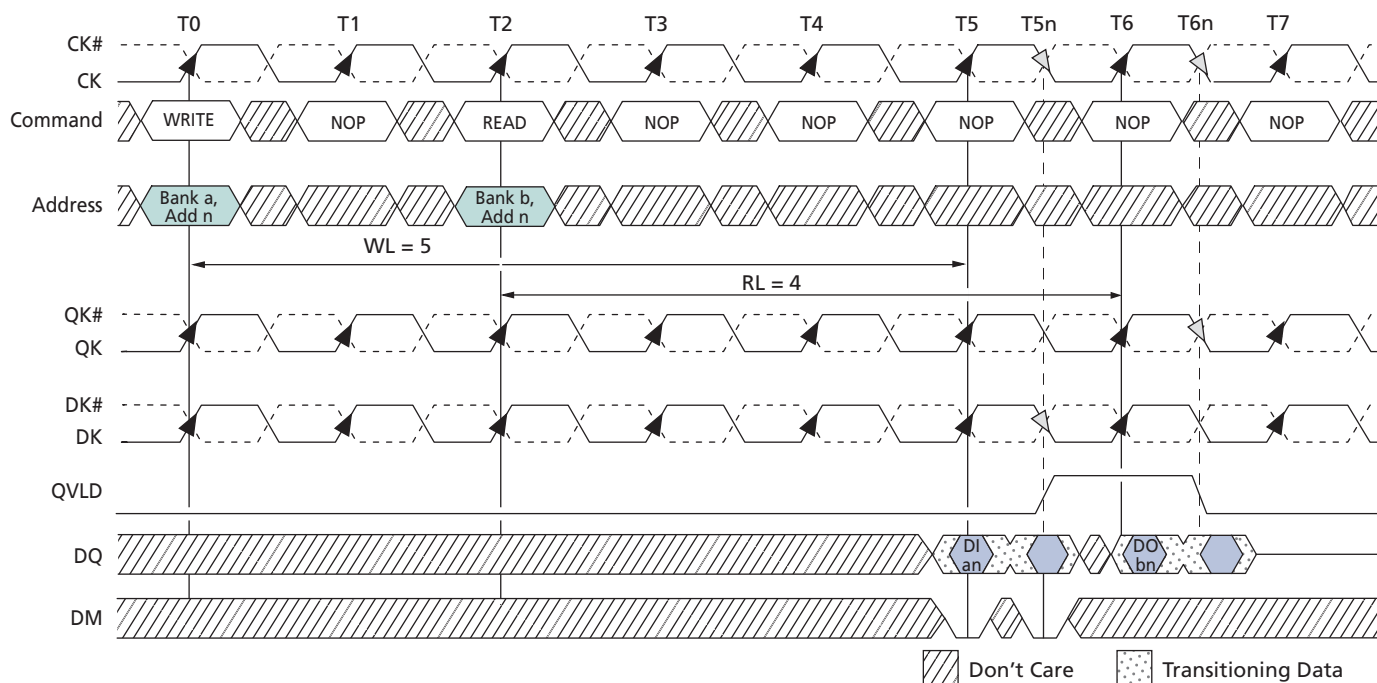
Figure 45: WRITE-to-READ
