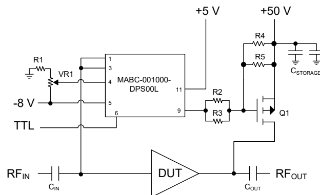
Figure 1. Fixed Gate/Pulsed Drain Biasing
