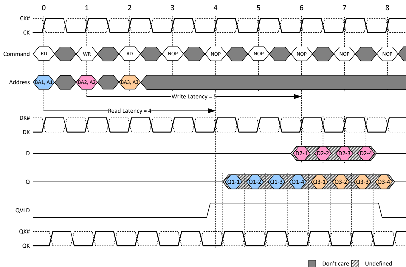
Read Followed by Write: BL = 4, RL = 4 &amp; WL = 5, Configuration 1
