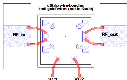
(a) Recommended Microstrip wire bonding
