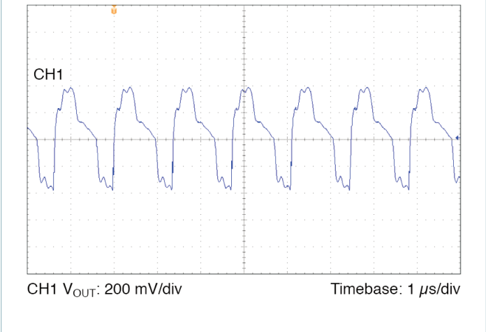
Figure 16 — Output voltage ripple, V_{IN} = 48\text{ V} , V_{OUT} = 36.0\text{ V} , C_{OUT\_EXT} = 220\text{ }\mu\text{F} , R_{LOAD} = 4.045\text{ }\Omega
