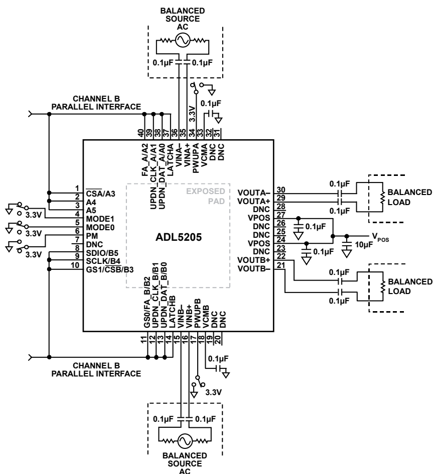
Figure 51. Basic Connections
