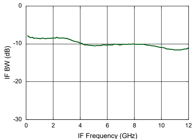
IF Bandwidth
