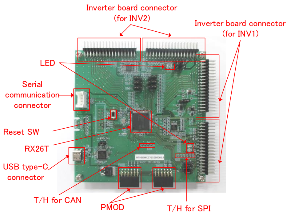
Figure 4-3 CPU Board Layout
