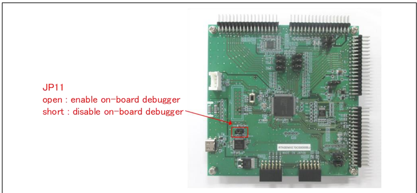
Figure 6-1 JP11 setting
