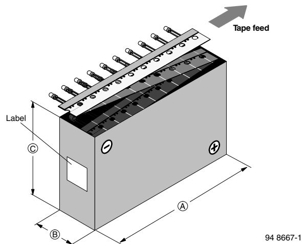
Fig. 21 - Tape Direction
