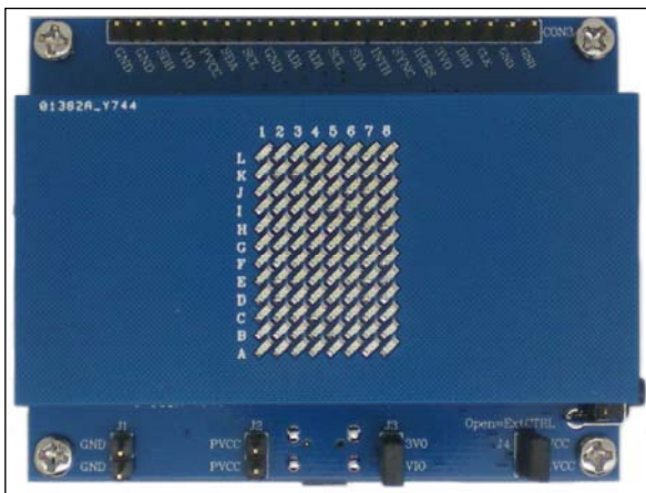
Figure 1: Photo of IS31FL3736B Evaluation Board
