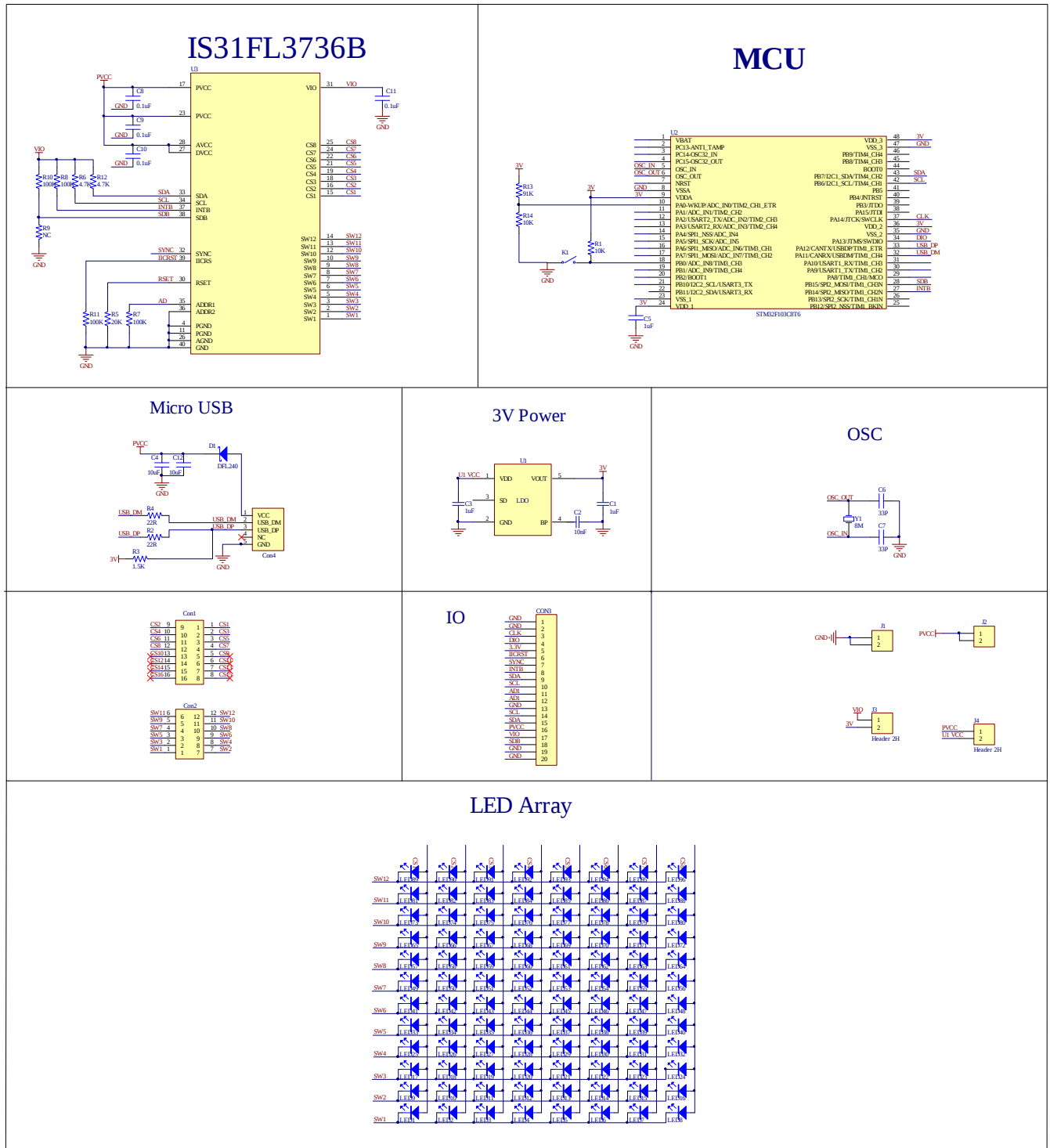
Figure 3: IS31FL3736B Application Schematic
