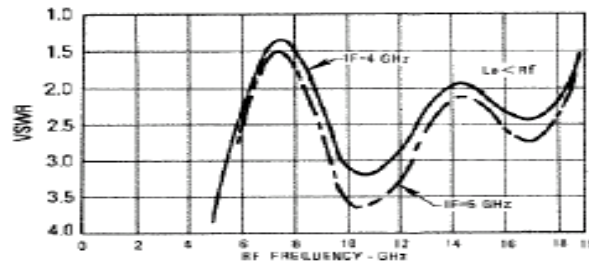
R-Port VSWR vs. Frequency
