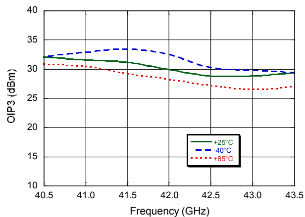
Output IP3 @ 2 GHz IF
