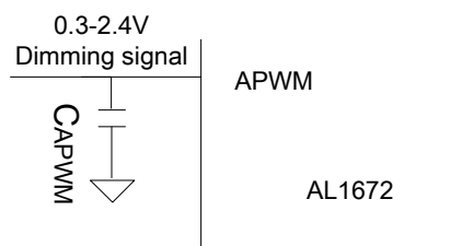
Figure 2: Analog Dimming Setting Circuit
