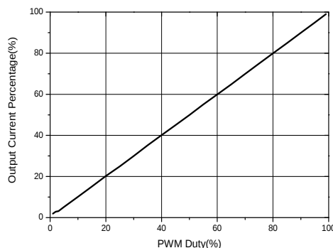
Figure 5: PWM Dimming Curve (PWM frequency is 1 KHz)
