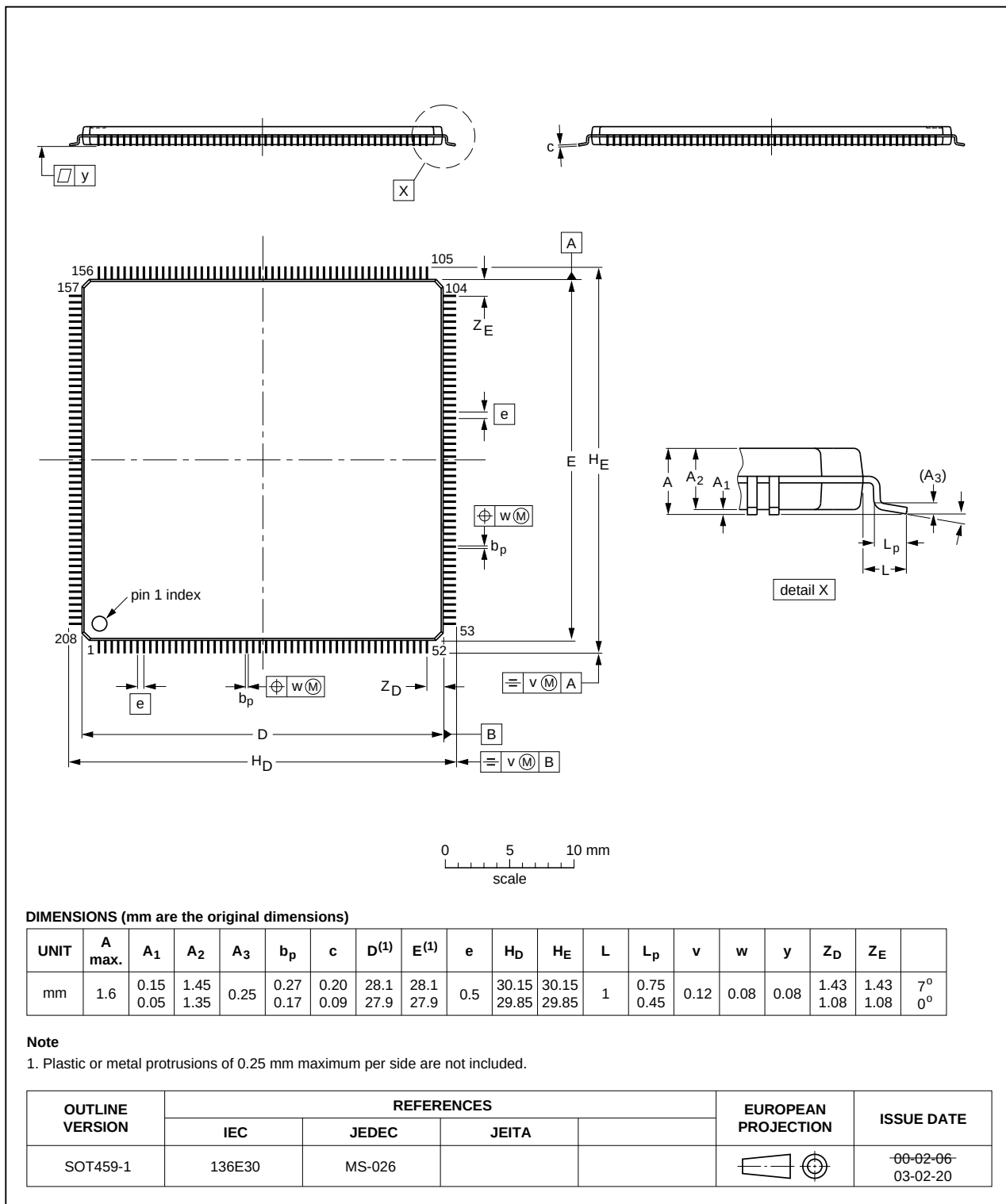
Fig 51. LQFP208 package
