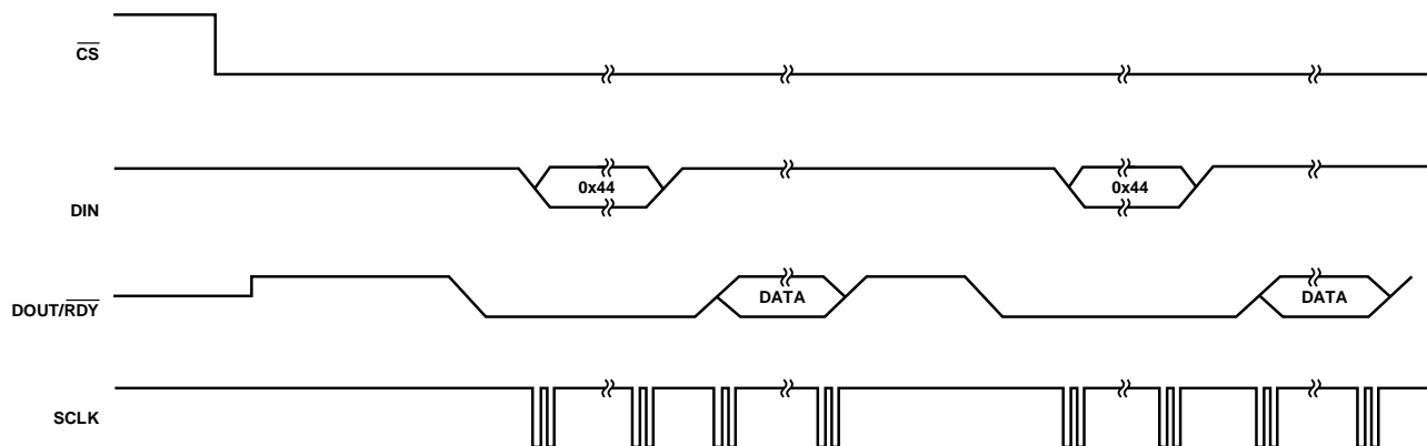
Figure 42. SPI Communication in Continuous Conversion Mode
