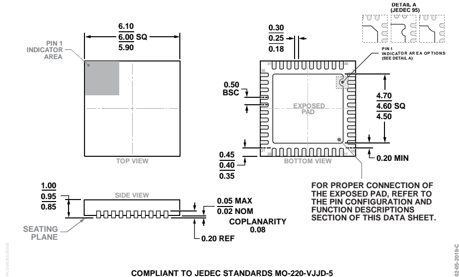
COMPLIANT TO JEDEC STANDARDS MO-220-VJJD-5 Figure 45. 40-Lead Lead Frame Chip Scale Package [LFCSP] 6 mm × 6 mm Body and 0.95 mm Package Height (CP-40-15) Dimensions shown in millimeters
