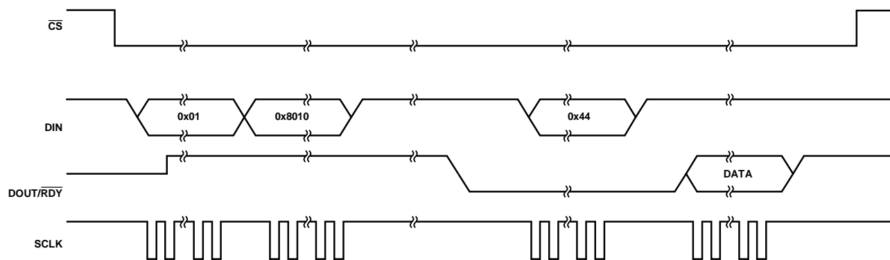
Figure 44. SPI Communication in Single Conversion Mode
