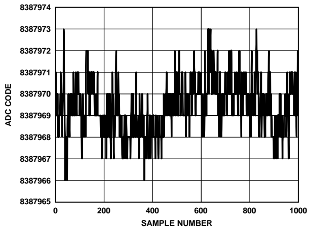
Figure 5. Noise (Output Data Rate = 2.5 SPS)
