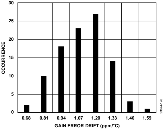
Figure 18. Gain Error Drift Distribution Histogram
