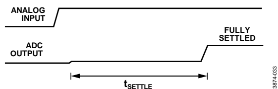
Figure 33. Step Input with Single Cycle Settling
