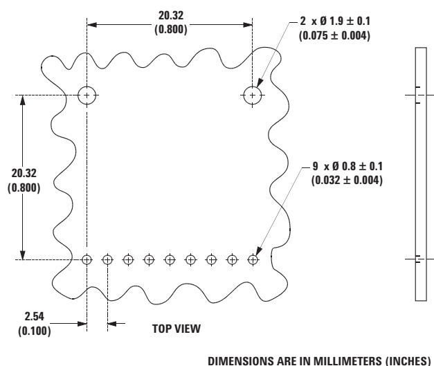
Figure 8a. Recommended Board Layout Hole Pattern
