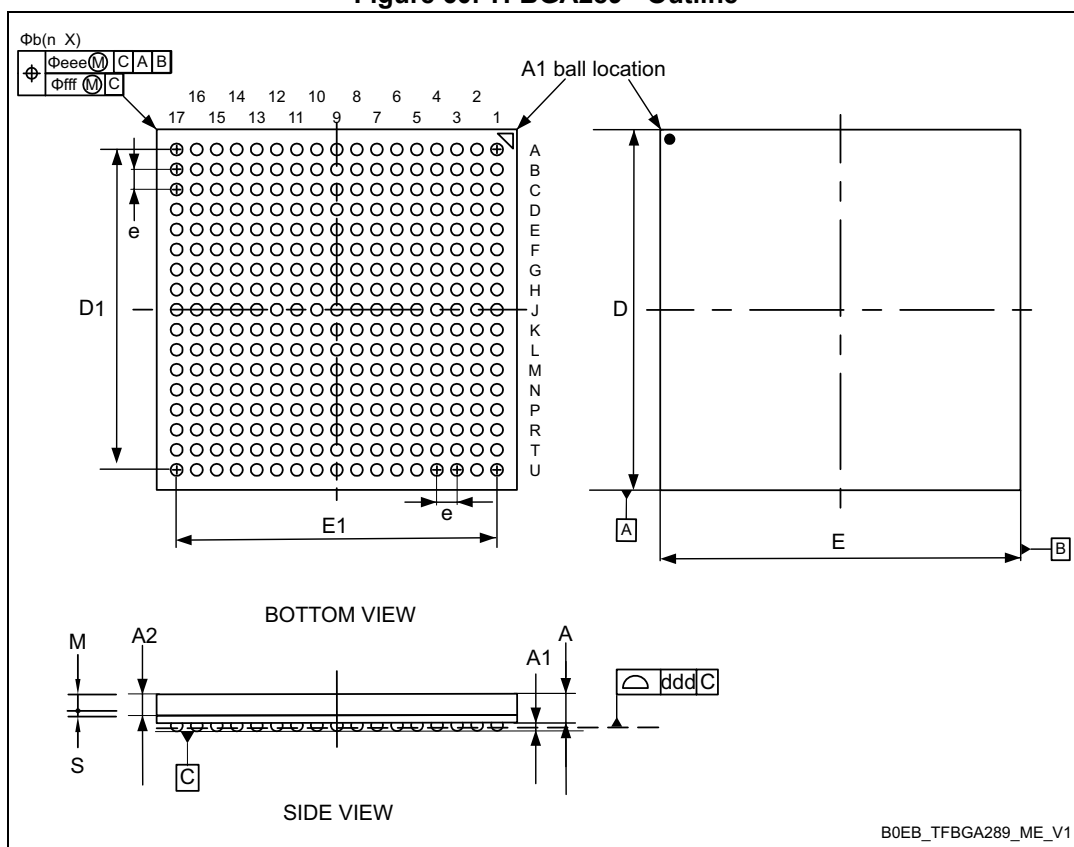
Figure 60. TFBGA289 - Outline
