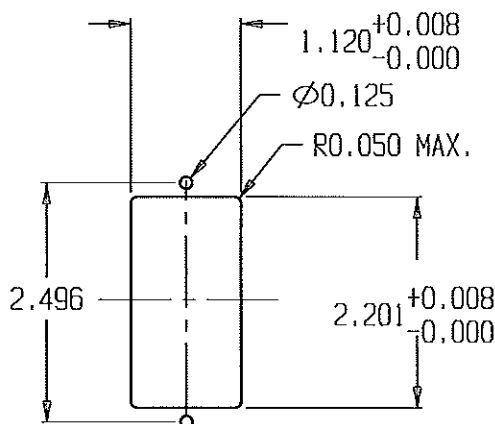
PANEL CUTOUT
