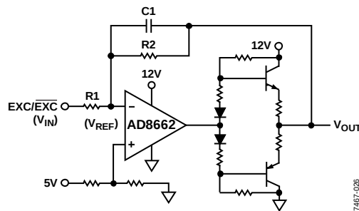
Figure 27. Buffer Circuit
