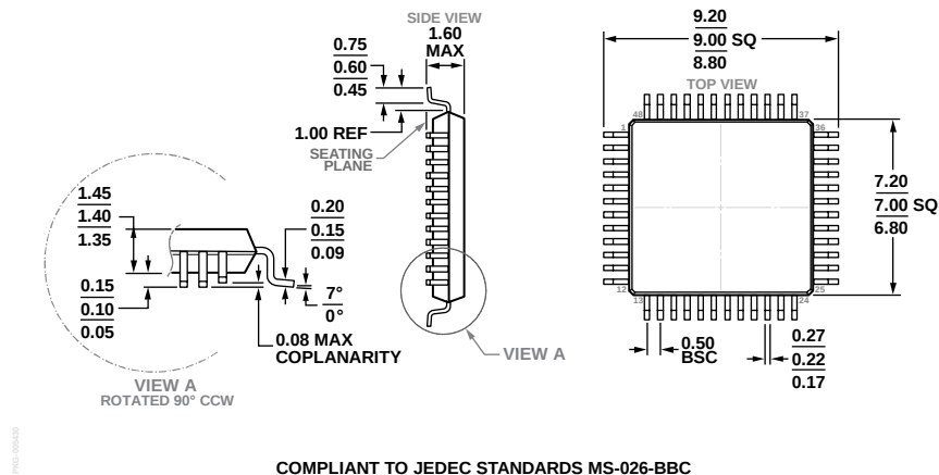
Figure 39. 48-Lead Low Profile Quad Flat Package [LQFP] (ST-48)
