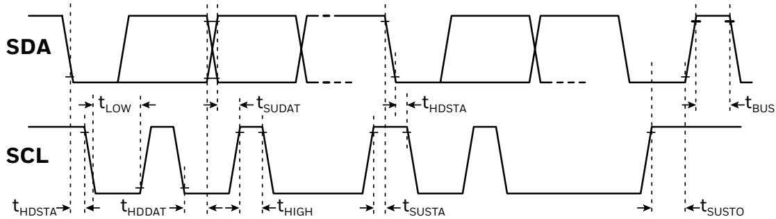
Figure 5. I 2 C Bus Timing Diagram and Parameters
