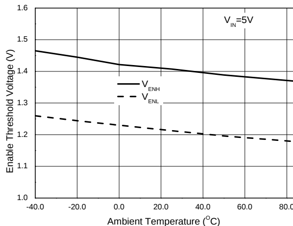
Enable Threshold Voltage vs. Ambient Temperature
